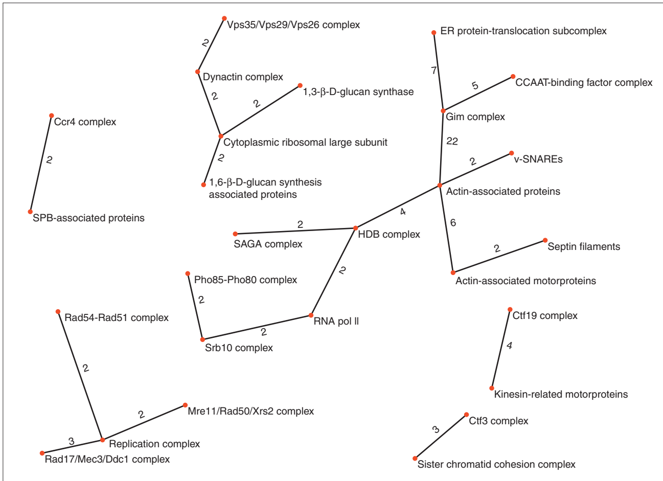
Figure 3 A thematic map of compensatory complexes. Here, nodes represent protein complexes, and a link is drawn between two nodes if there is a significantly large number of inter-complex SSL interactions. Links between compensatory complexes are labeled with the numbers of supporting SSL interactions.
