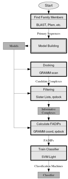
(b) Creating the Classifier
